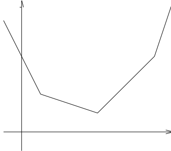
Figure 2: A convex piecewise linear function.
