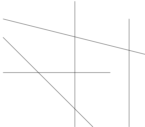
Figure 1: An arrangement of lines.
