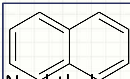
Naphthalene
