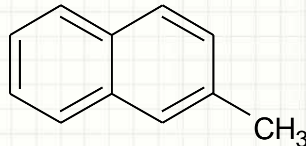
2-methyl naphthalene
