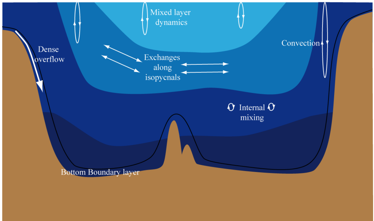
Figure 3.6: Schematic representation of some small-scale processes that have to be parameterized in ocean models. Modified from http://www.gfdl.noaa.gov/ocean-models-at-gfdl .
