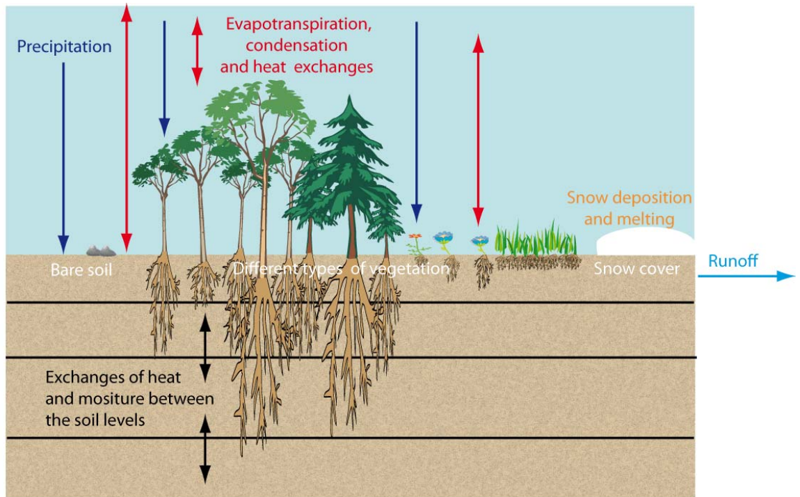
Figure 3.8: The main processes that have to be taken into account in a land surface model. For clarity, the carbon storage in plants and in soils, as well as the exchanges between these reservoirs and with the atmosphere are not shown.
