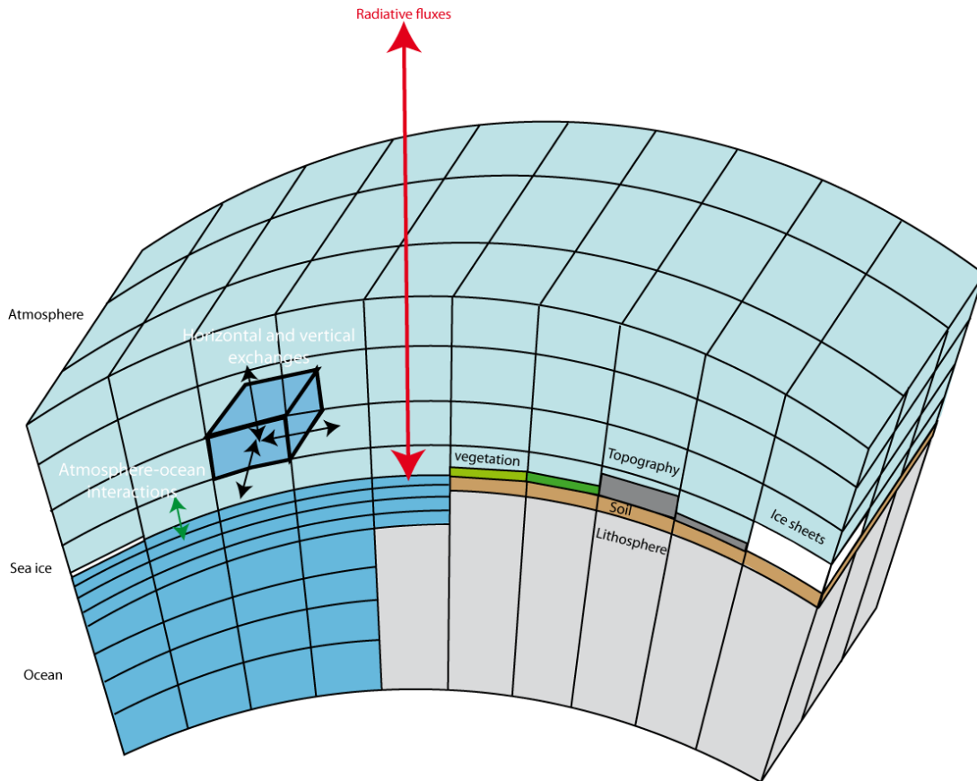
Figure 3.5: A simplified representation of part of the domain of a general circulation model, illustrating some important components and processes. For clarity, the curvature of the Earth has been amplified, the horizontal and vertical coordinates are not to scale and the number of grid points has been reduced compared to state-of-the-art models.
