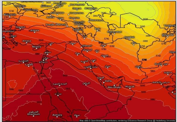
Geopotential height, 500hPa (m) Valid for Wed 05/13/2020, 11:00pm GMT+03 Middle East GFS (15 days) from 05/13/2020/12z meteo1gix.com
