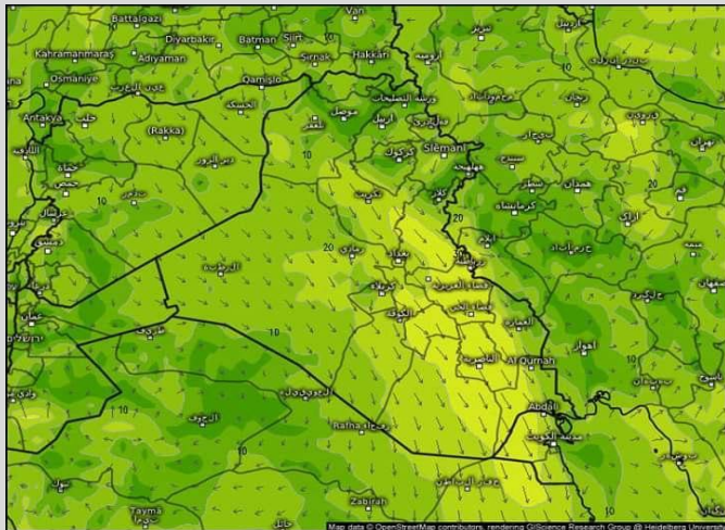
Wind direction and mean wind speed (kph) Valid for Thu 05/14/2020, 02:00pm GMT+03 Iraq GFS (15 days) from 05/13/2020/12z meteo1gix.com
