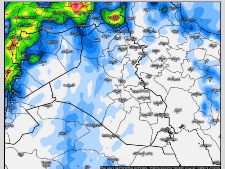
Precipitation, 24h (mm) Sun 05/24/2020, 08:00pm GMT+03 Valid for Sun 05/24/2020, 08:00pm GMT+03 Iraq GFS (15 days) from 05/21/2020/12Z meteoqlix.com
