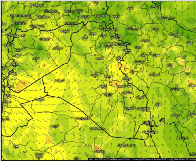
Wind direction and mean wind speed (kph) Sun 05/24/2020, 05:00pm GMT+03 Valid for Sat 05/23/2020, 03:00am GMT+03 Iraq GFS (15 days) from 05/21/2020/12Z meteoqlix.com
