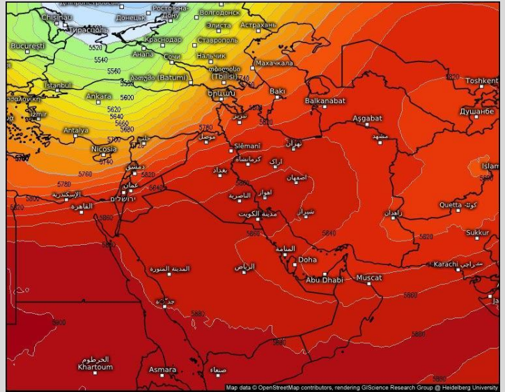
Geopotential height, 500hPa (m) Sat 05/23/2020, 03:00am GMT+03 Valid for Sat 05/23/2020, 03:00am GMT+03 Middle East GFS (15 days) from 05/21/2020/12Z meteoqlix.com
