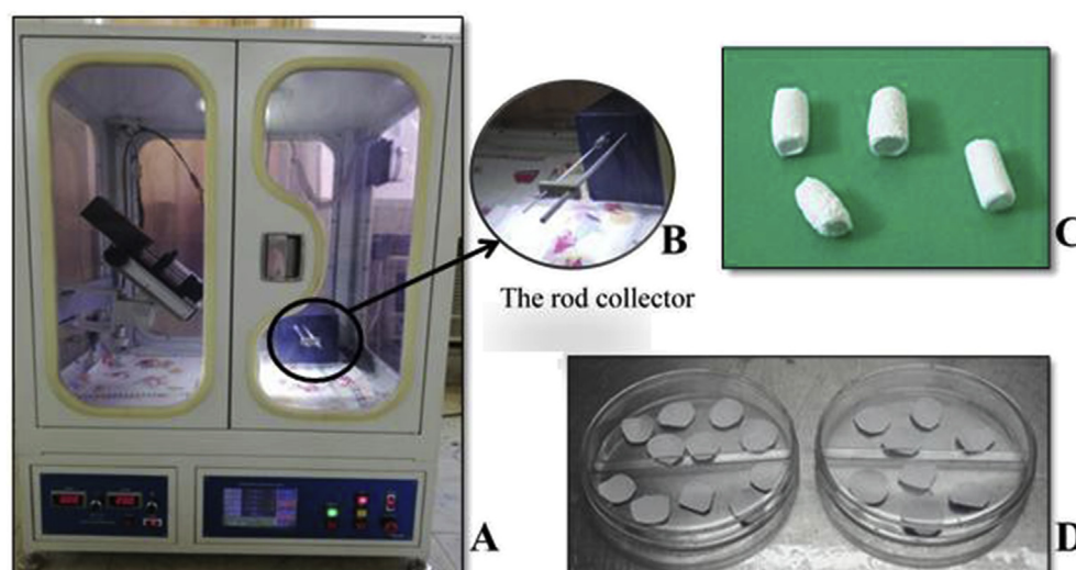
Figure 3: A) Bio-Electrospinning/Electrospray system, B) Rod collector for scaffold shaping, C) Cylindrical PCL scaffold, D) Discs PCL scaffold.
