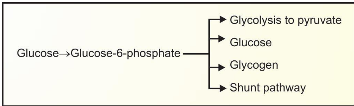
Fate of glucose 6- phosphate
