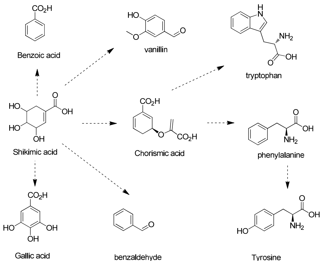
Figure 4: Shikimate pathway
