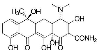
Figure 3: tetracycline
