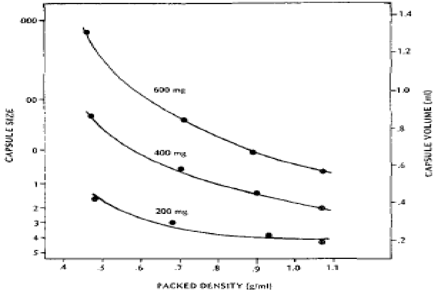
FIG. 8-15. Correlation between capsule size and packed density for different fill weights (200–600 mg).
