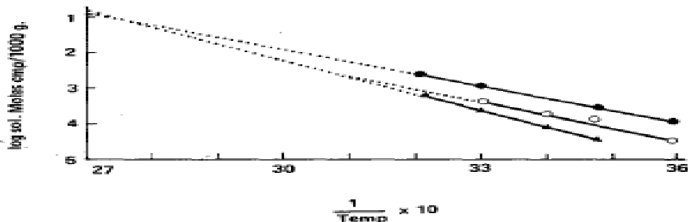
FIG. 8-14. The van't Hoff plot of solubility vs. reciprocal absolute temperature for polymorphs A, B, and C of chloramphenicol palmitate. Key: Polymorphs A ( \blacktriangle ); B ( \bullet ); and C ( \circ ). (From Aguiar, A. J., et al.: J. Pharm. Sci. , 58:983, 1969. Reproduced with permission of the copyright owner.)
