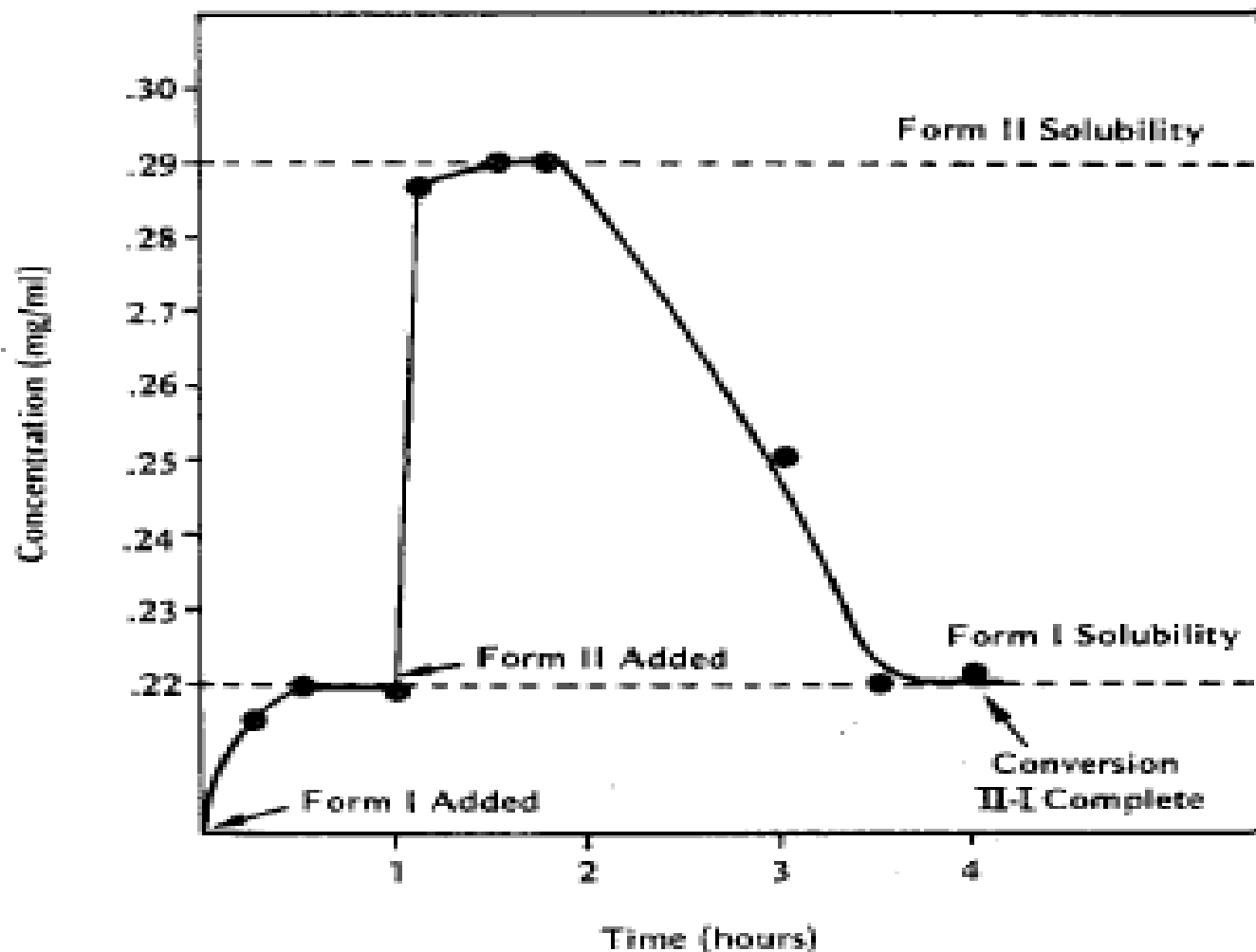
FIG. 8-21. Powder dissolution profiles for two polymorphic forms of an organic acetate salt in acetonitrile at 25°C.
