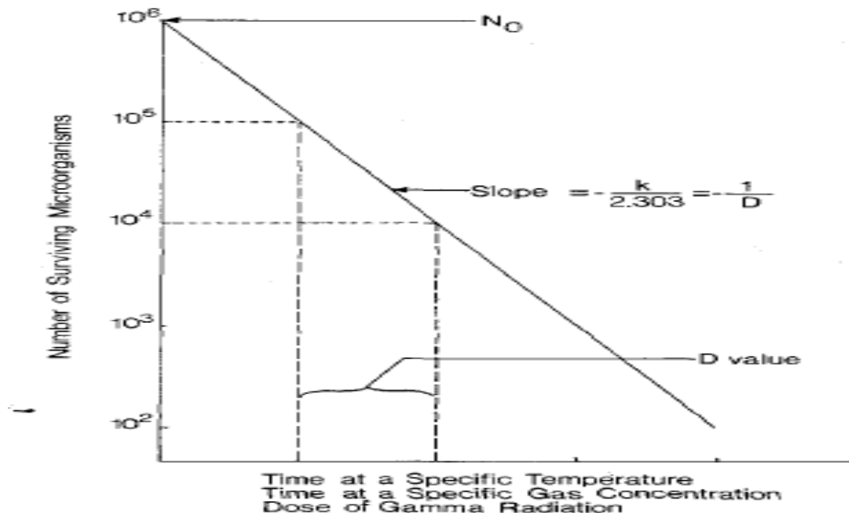
FIG. 21-1. Graphic representation of the semilogarithmic microbial death rate.
