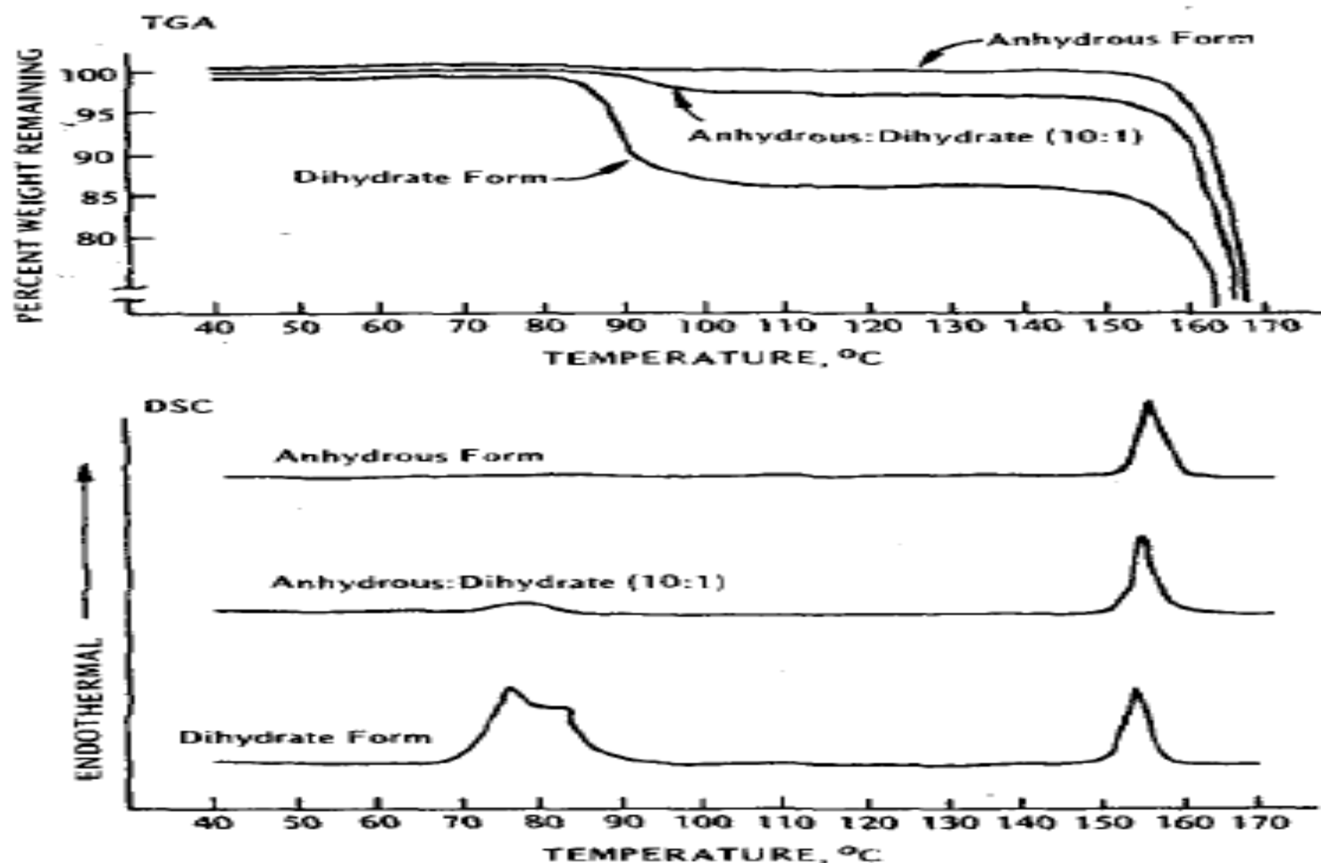
FIG. 8-11. Thermogravimetric (TGA) and differential scanning calorimetric (DSC) analysis for an acetate salt of an organic amine that has two crystalline forms, anhydrous and dihydrate. Anhydrous/dihydrate mixture was prepared by dry blending. Heating rate was 5°/min.
