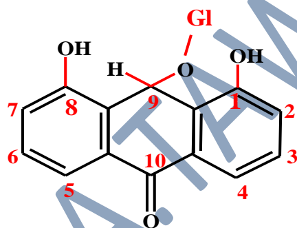
Emodin-oxanthrone-9-glucoside
