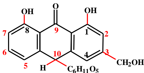
1,8-Dihydroxy- 3-hydroxymethyl-9-anthrone-10-glucoside
