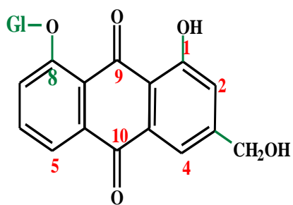
Aloe-emodin-8-glycoside
