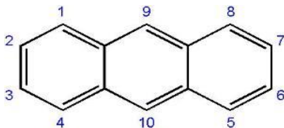
Anthracene
