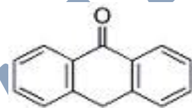
anthrone
