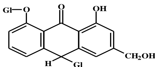
Cascaroside A & B
