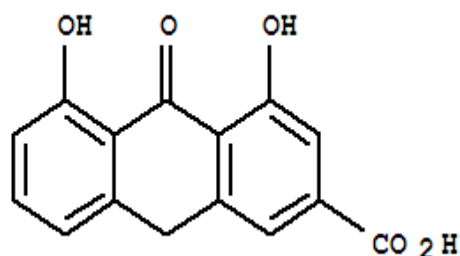
Images of rhein & rhein anthrone
