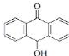
oxanthrone
