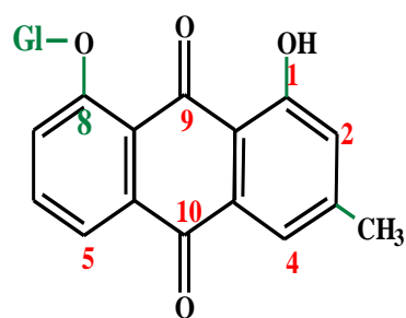
Chrysophanol-8-glycoside
