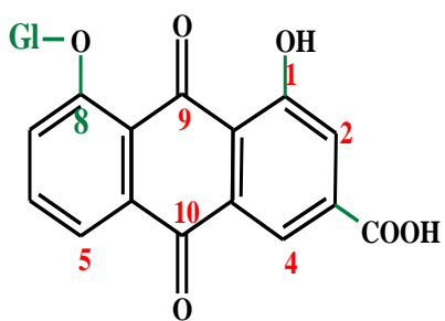
Rhein-8-glycoside
