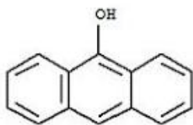
Anthranol
