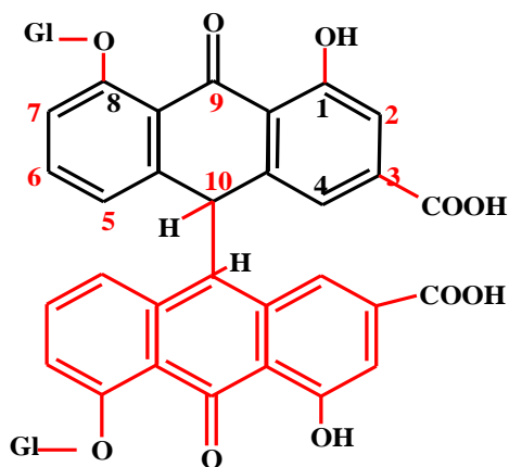
Sennoside A&B
