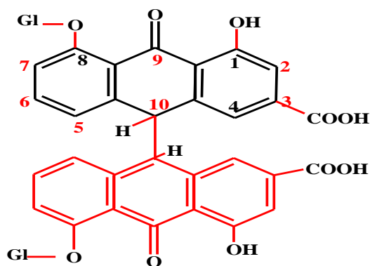
Sennoside A&B
