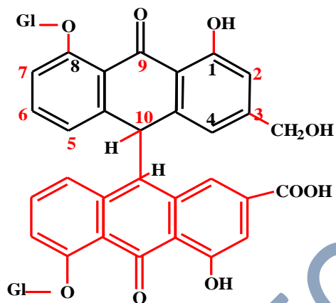
Sennoside C&D
