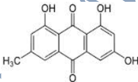
Emodin
