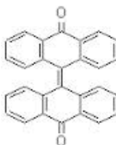
dianthrone
