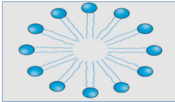
Diagrammatic cross-section of a micelle.
