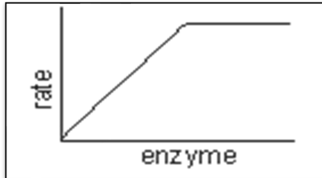
Enzyme concentration affect on rates of reaction
