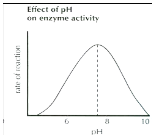
Effect of pH affect on rates of reaction
