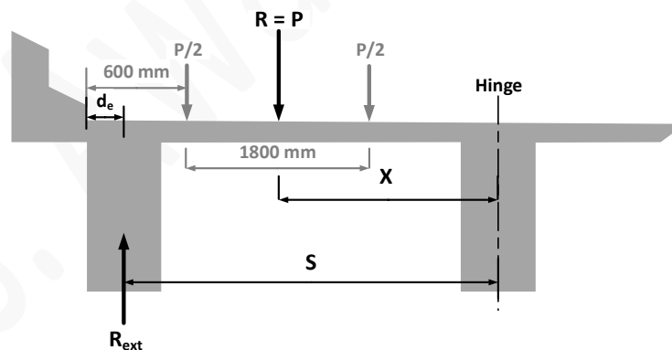
Lever Rule for Exterior Beam
