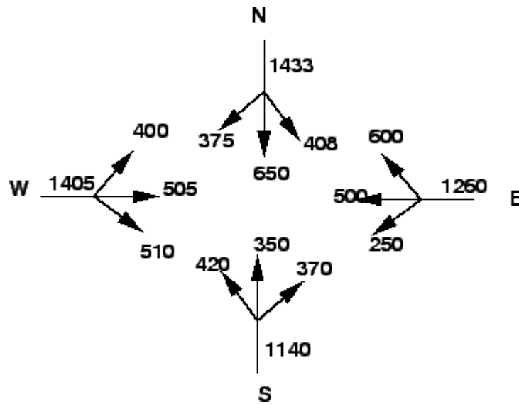
Figure : Traffic approaching the rotary
