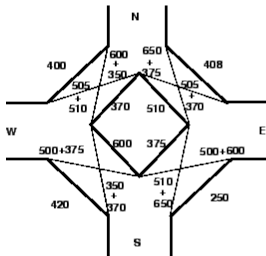
Figure : Traffic negotiating a rotary
