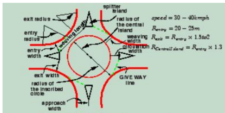
Figure: Design elements of a rotary.
