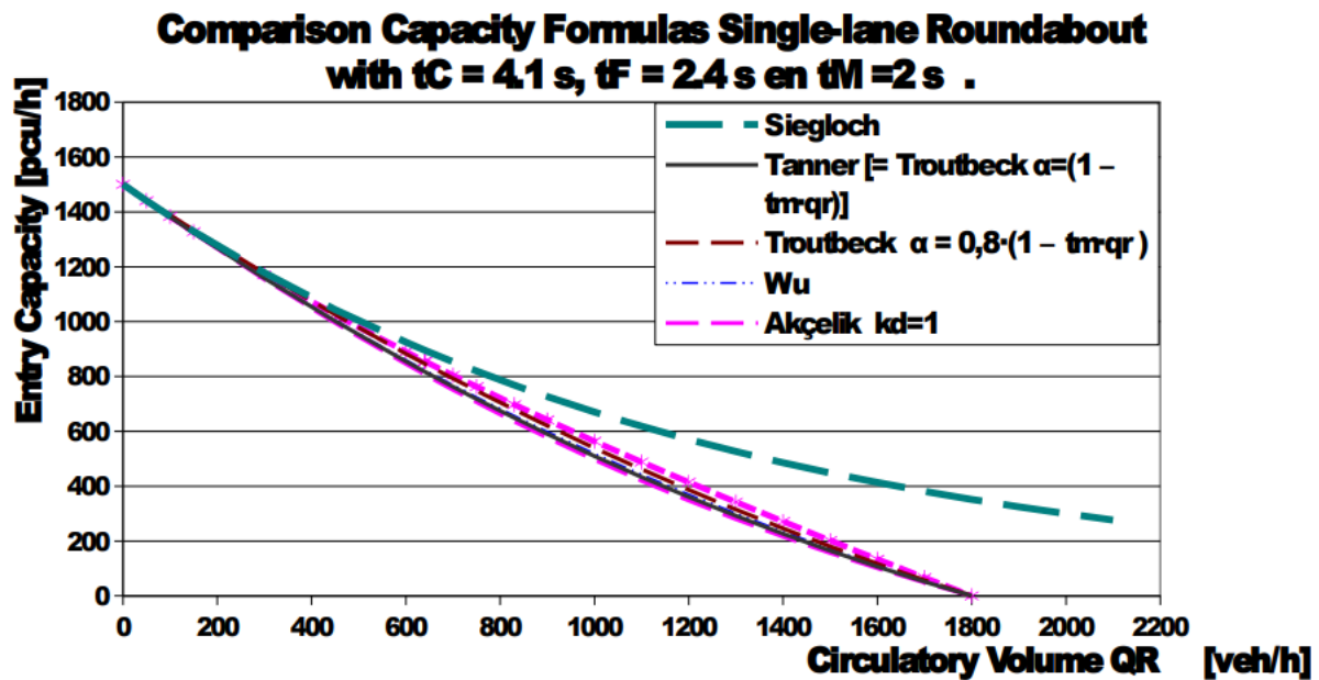
Figure 8: The inflow onto a road (or roundabout) as function of the main road (roundabout) traffic – figure from Fortuijn and P. (2015)
