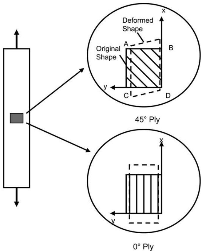
Fig. 1.7 Shear coupling in a 45° ply. Source: Ref 1
