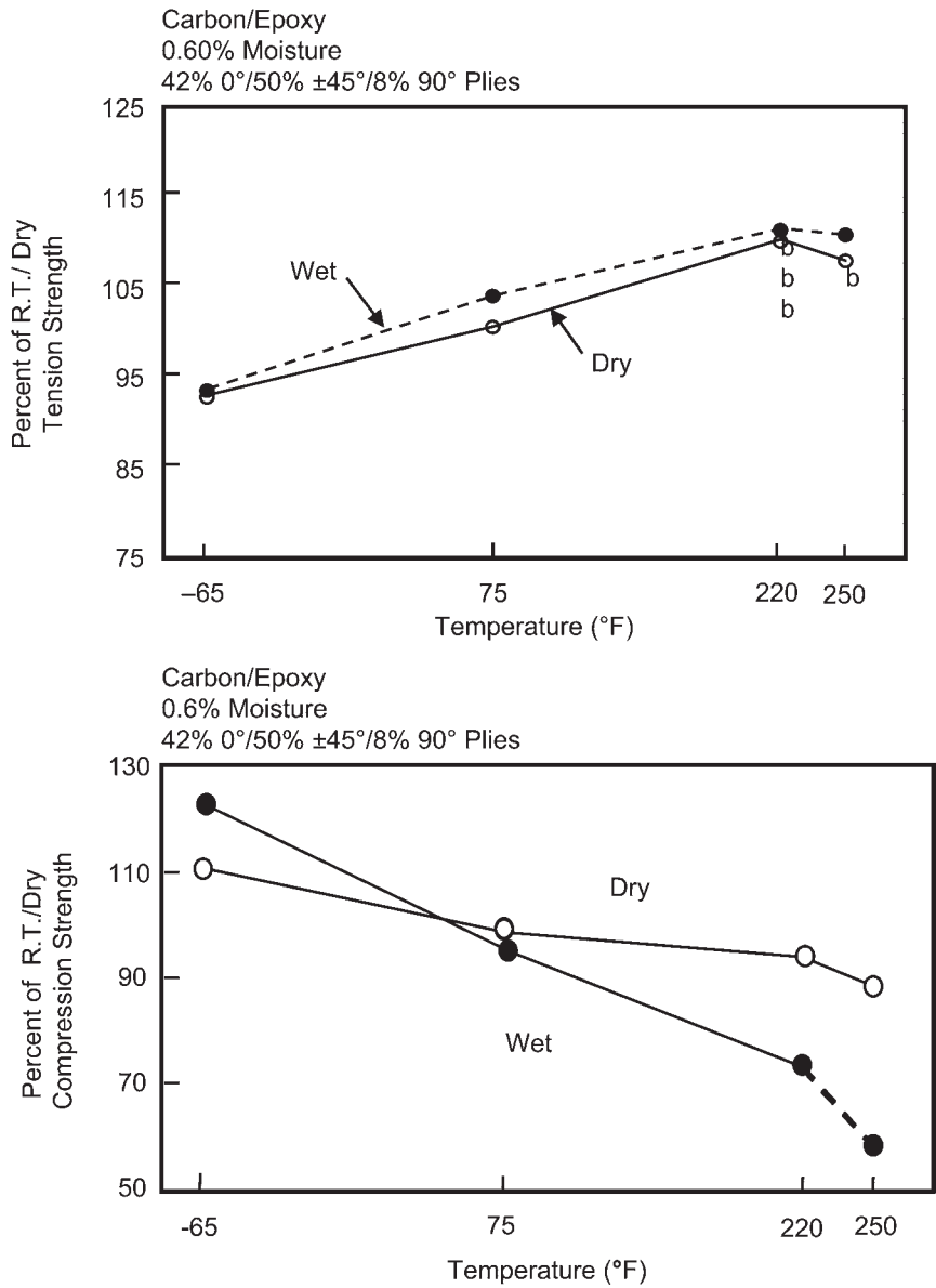
Fig. 1.22 Effects of temperature and moisture on strength of carbon/epoxy. R.T., room temperature
