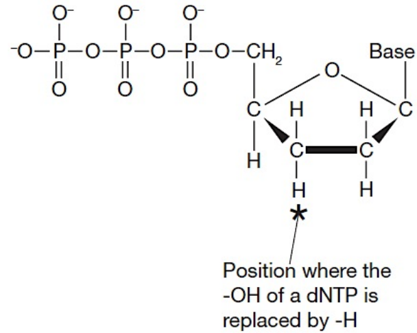
(c) Strand synthesis terminates when a ddNTP is added
