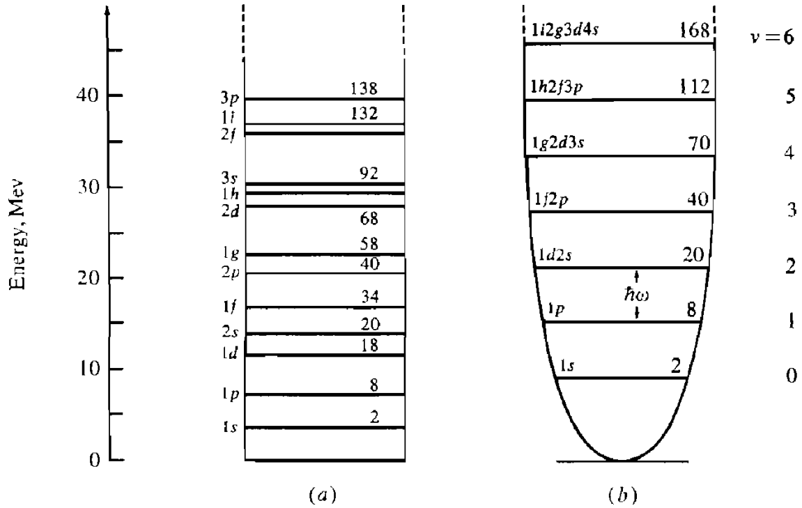
Figure (3-4): Energy levels of nucleons. (a) in an infinite spherical square-well potential. (b) in a harmonic oscillator potential. The spectroscopic notation (n, \ell) and the total occupation number up to any particular level are given.
