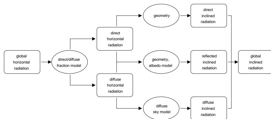
Fig. 6.1. Conversion steps for estimating global radiation on tilted surfaces from global horizontal radiation.
