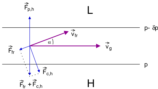
Fig. 13.3. The balance of horizontal forces in the atmospheric boundary layer. The pressure gradient force F_{p,h} is balanced by the sum of the Coriolis force F_{c,h} and the friction force F_{fr} .
