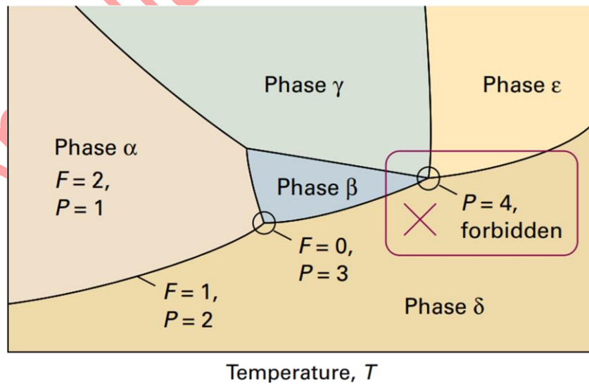
Figure 1-1: The typical regions of a one-component phase diagram. The lines represent conditions under which the two adjoining phases are in equilibrium. A point represents the unique set of conditions under phases coexist in equilibrium. Four phases cannot mutually coexist in equilibrium when only component is present.
