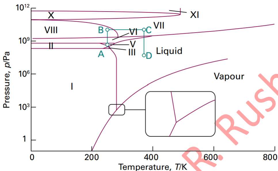
Figure 1-2: The phase diagram for water showing
