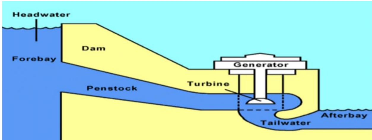
Fig.8-1 Dam scheme
