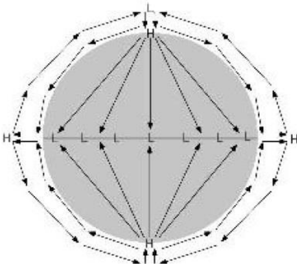
Figure 3.2: Simplified one-cell global air circulation patterns.
