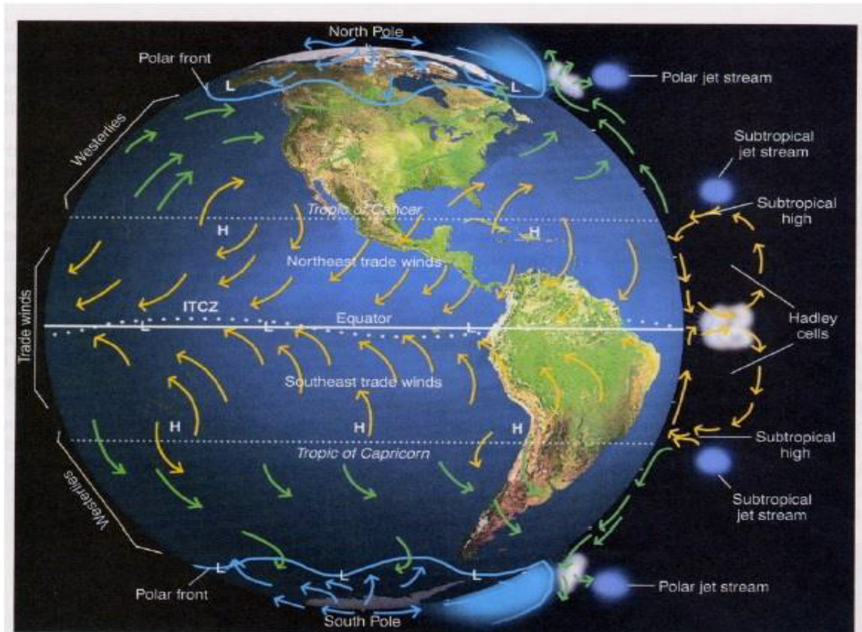
Figure 3.3: General circulation schematic.
