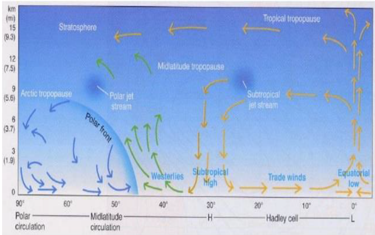
Figure 3.4: Equator-to-pole cross section of the Northern Hemisphere. It shows the Hadley cell, subtropical highs, the subpolar low-pressure cell, and approximate locations of the subtropical and polar jet streams.
