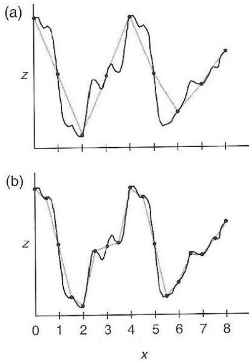
Figure 1. The effect of increasing the number of grid points
