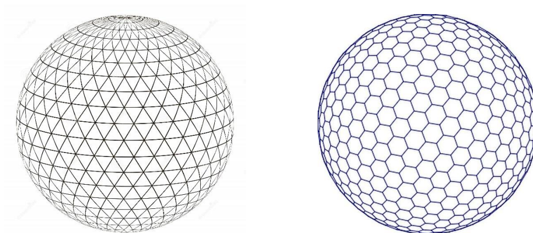
Figure 2. Examples of rectangular or latitude-longitude grid, triangular grid and hexagonal grid.
