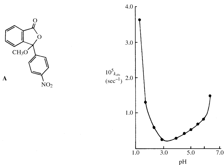
Fig. 8.P21. pH–Rate profile for hydrolysis of A in buffered aqueous solution at 70^\circ\text{C} .
