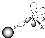
stabilizing interaction with \sigma^*
