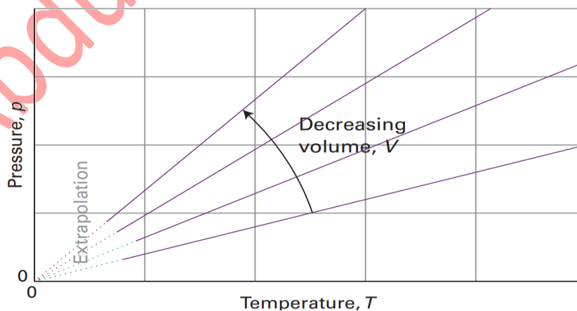
Figure 3: The pressure also varies linearly with the temperature at constant volume, and extrapolates to zero at T = 0 ( -273 \text{ }^\circ\text{C} ).
