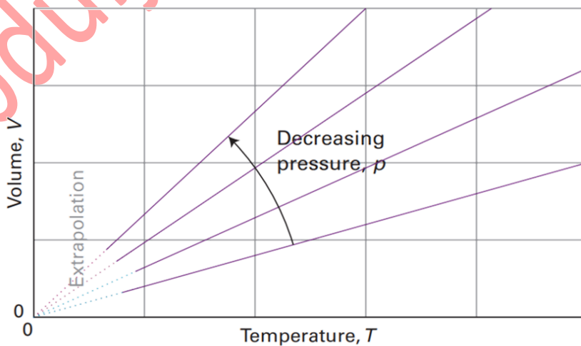
Figure 2: The variation of the volume of a fixed amount of gas with the temperature at constant pressure. Note that in each case isobars extrapolate to zero volume at T = 0 , or -273 \text{ OC}
