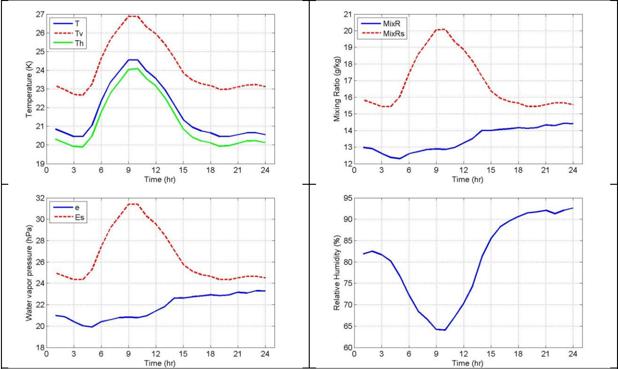
Fig 3. Air properties for rainy day (28 Oct 2015)
