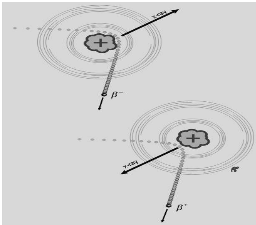
Figure (5-1): Bremsstrahlung. Beta particles ( \beta^- ) and positrons ( \beta^+ ) that travel near the nucleus will be attracted or repelled by the positive charge of the nucleus, generating x-rays in the process.
