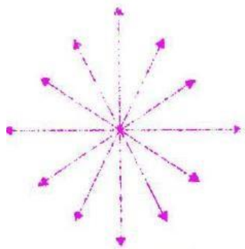
Figure (9) Schematic representation of partially polarized light.
