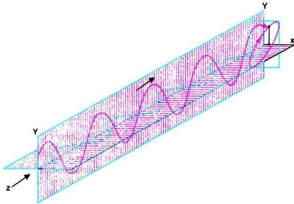
Figure (10) Elliptically polarized light is produced when two orthogonal coherent waves having different amplitudes and a phase difference of 90^\circ , superpose on each other.
