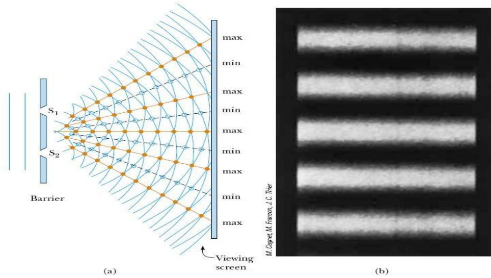
Figure (4). (a) Schematic diagram of Young's double-slit experiment. Slits S1 and S2 behave as coherent sources of light waves that produce an interference pattern on the viewing screen (drawing not to scale). (b) An enlargement of the center of a fringe pattern formed on the viewing screen.
