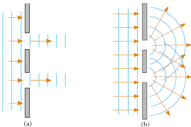
Figure (3). (a) If light waves did not spread out after passing through the slits, no interference would occur. (b) The light waves from the two slits overlap as they spread out, filling what we expect to be shadowed regions with light and producing interference fringes on a screen placed to the right of the slits.
