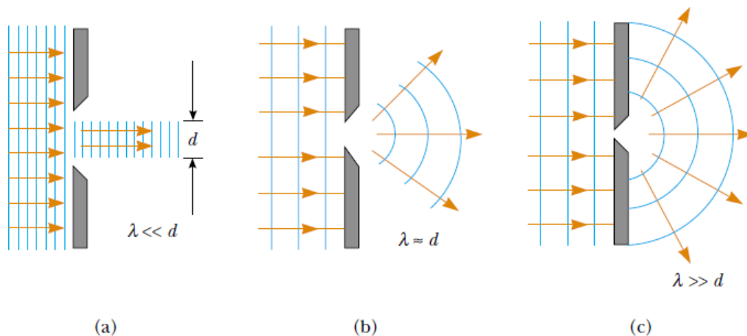
Figure (6). A plane wave of wavelength \lambda is incident on a barrier in which there is an opening of diameter d . (a) When \lambda \ll d , the rays continue in a straight-line path and the ray approximation remains valid. (b) When \lambda \approx d , the rays spread out after passing through the opening. (c) When \lambda \gg d , the opening behaves as a point source emitting spherical waves.
