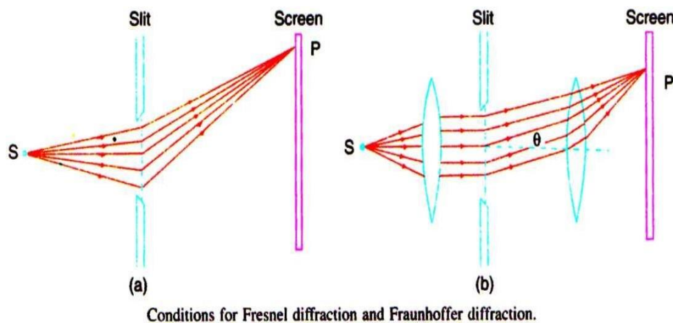
Figure (7) Conditions for Fresnel diffraction and Fraunhofer diffraction.
