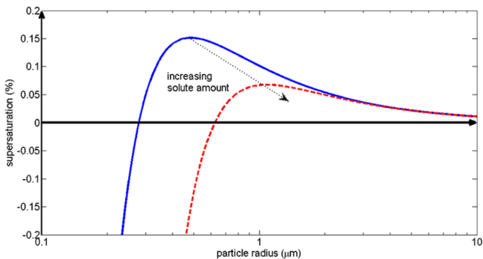
Figure 2: Köhler curve for two drops: m_s = 1 \times 10^{-17} g (blue solid line), m_s = 5 \times 10^{-17} g (red dashed line).
