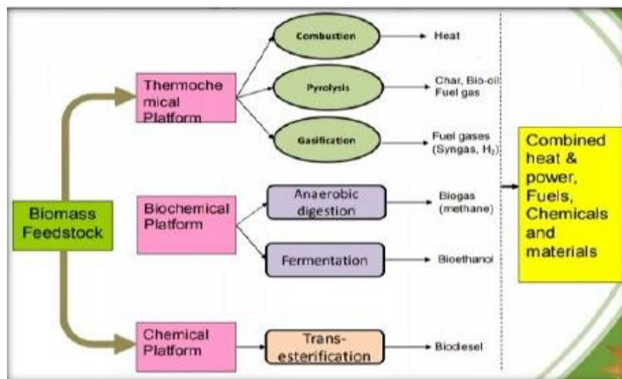
Figure 4: Bioenergy Production Routes
