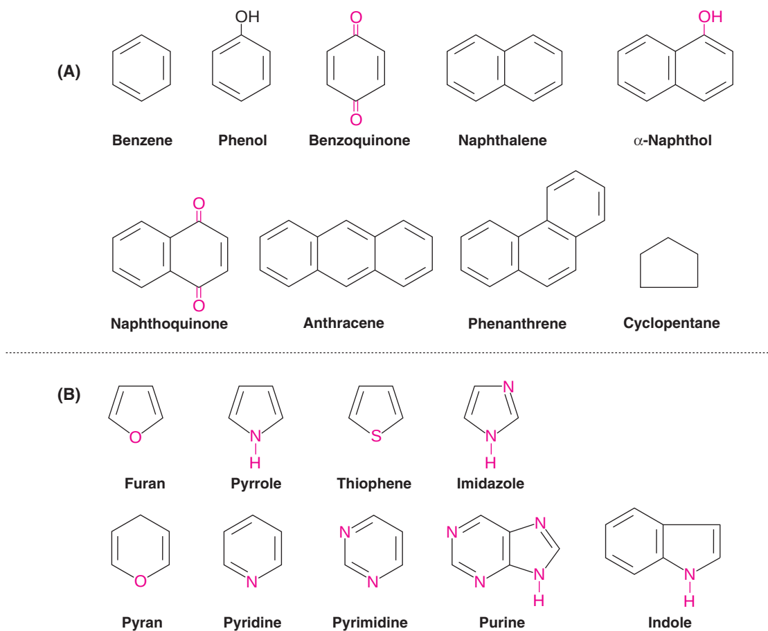
Fig. 39.1 : Common ring structures found in biomolecules (A) Homocyclic rings (B) Heterocyclic rings.
