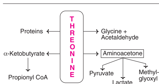
Fig. 15.42 : Overview of threonine metabolism.
