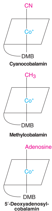
Fig. 7.36 : Coenzyme derivatives of vitamin B 12 (Note : Corrin ring represented diagrammatically is identical in all; DMB-Dimethylbenzimidazole).
