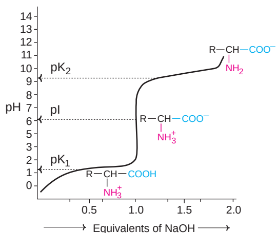
Fig. 4.3 : Titration curve of an amino acid-leucine (\text{R} = (\text{CH}_2)_2-\text{CH}-\text{CH}_2-) \text{pK}_1 = \text{Dissociation constant for COOH} ; \text{pI} = \text{Isoelectric pH} ; \text{pK}_2 = \text{Dissociation constant for NH}_3^+ .
