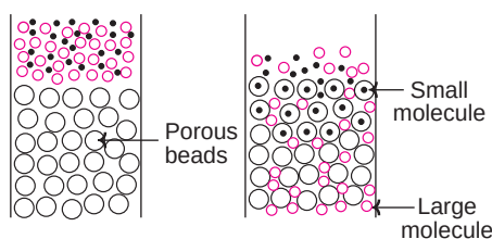
Fig. 41.6 : The principle of gel-filtration chromatography.
