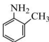
O-Toluidine O-methyl aniline
