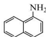
Naphthyl amine
