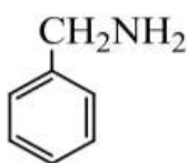
Benzyl amine
