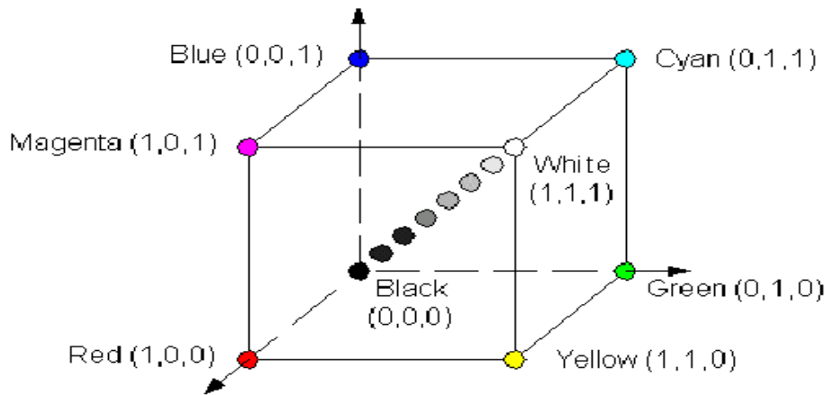
RGB 24-bit color cube
